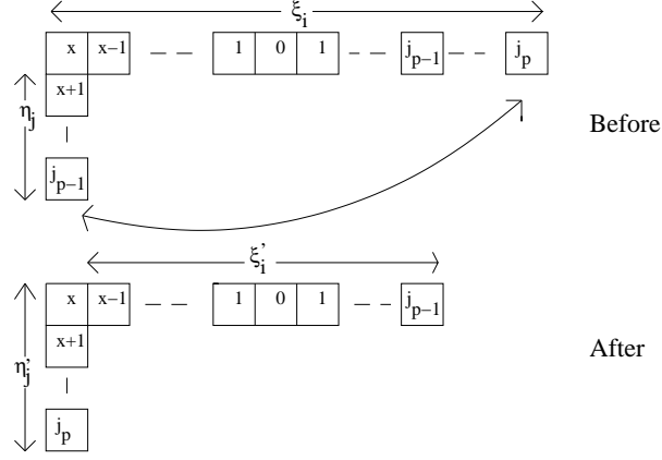
FIGURE 6. Example of flip
